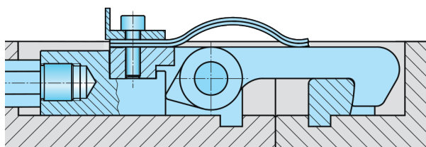
Transport position
