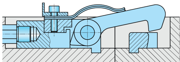
Production position
